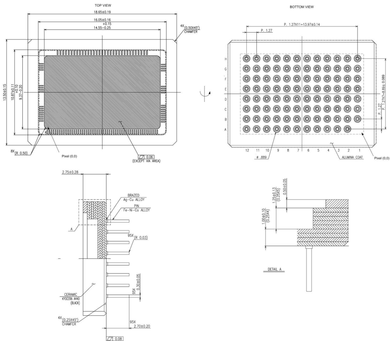
Figure 39: Package drawing of the CMV2000. All distances in mm.
