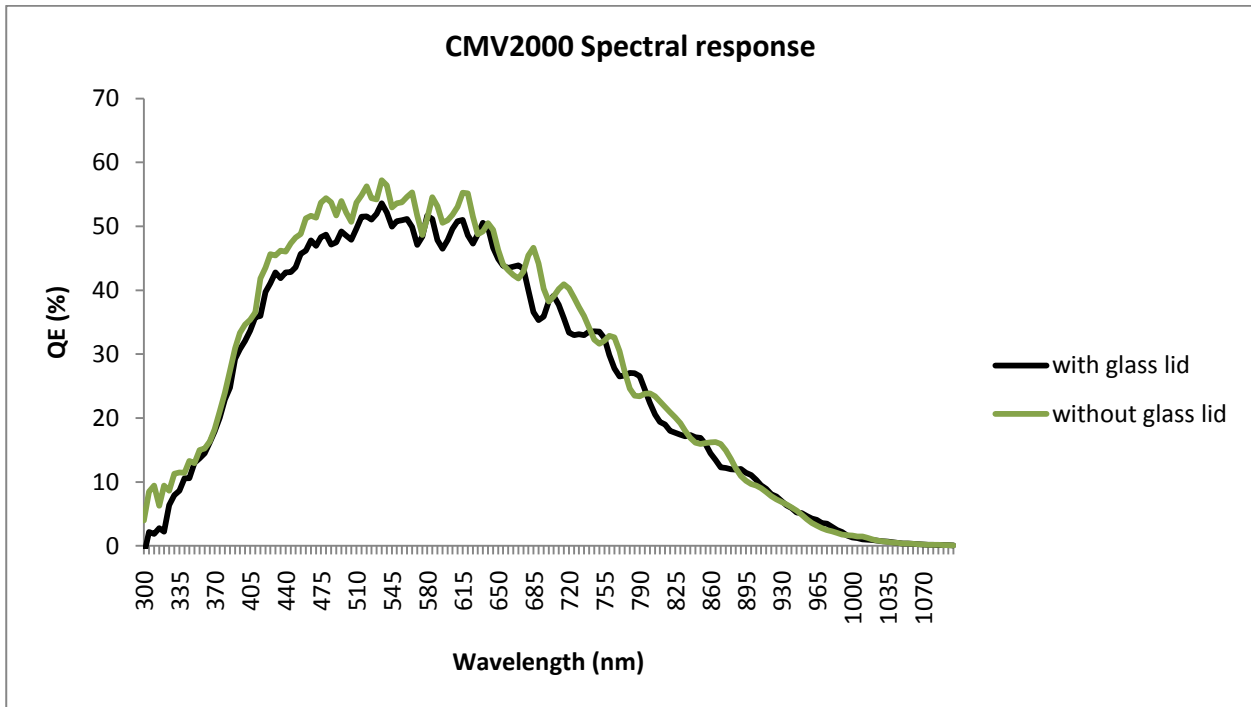
Figure 43: Typical spectral response of the CMV2000
