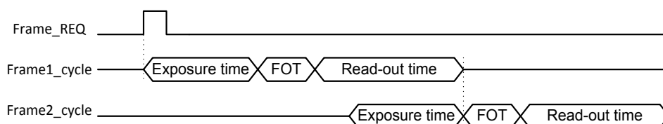
Figure 12: Request for 2 frames in internal exposure mode with exposure time < read-out time
