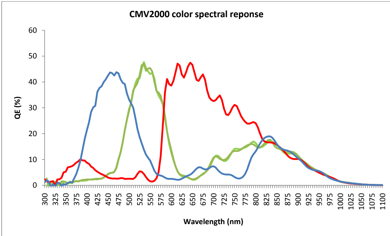
Figure 42: Typical spectral response of CMV2000 with RGB color filters and D263 cover glass
