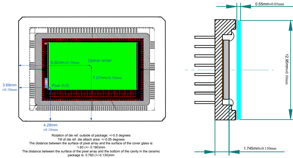
Figure 40: Assembly drawing of CMV2000.
